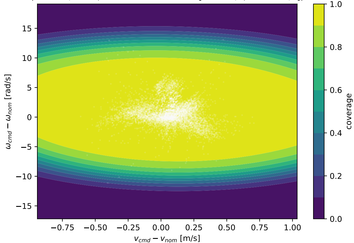
Residual coverage vs command offset (0 = off / OOD; state fixed at mean [0.54 m/s, 0.50 rad/s])
